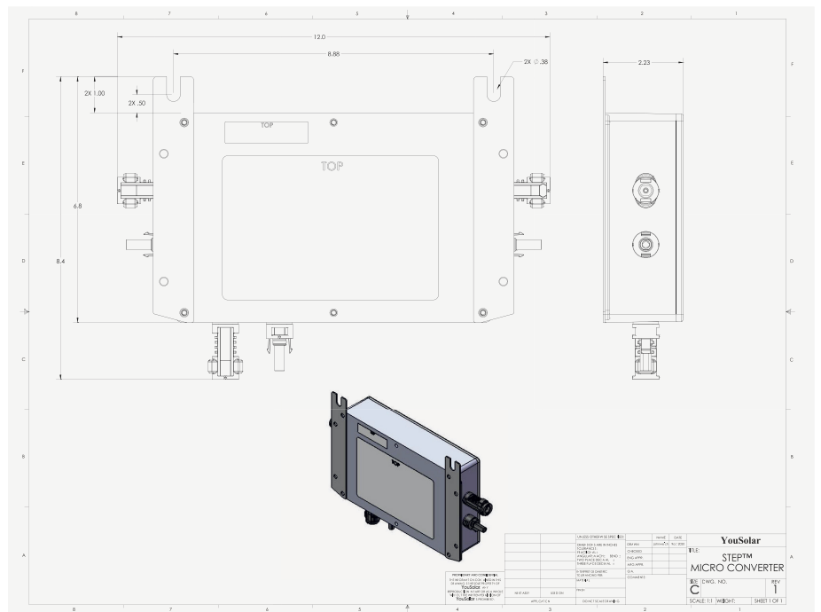
The drawing of the exterior design of STEP which shows its attachment point.
